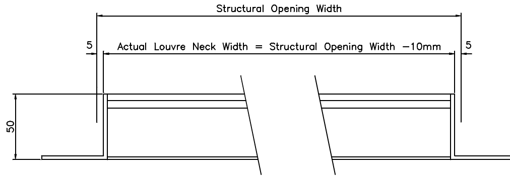
Sectional Plan On Arrow B.B.
