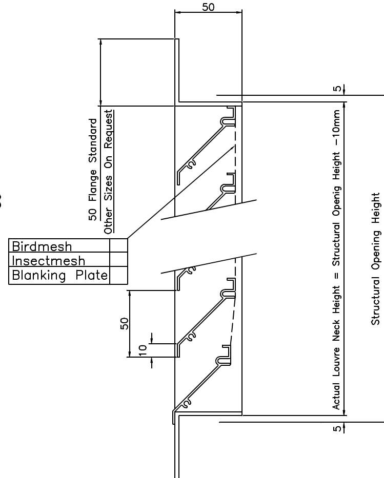
Sectional Elevation On Arrow A.A.
