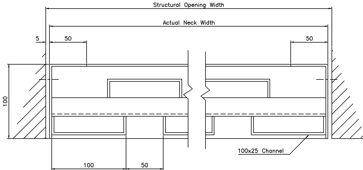
Sectional Plan At Jamb
