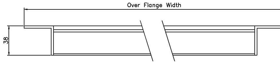
Sectional Plan On Arrow B.B.
