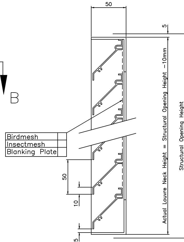
Sectional Elevation On Arrow A.A.
