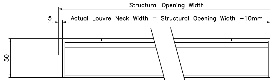
Sectional Plan On Arrow B.B.
