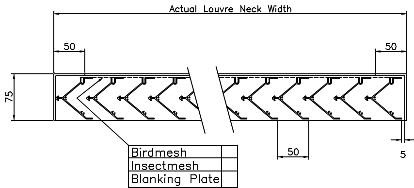
Sectional Plan On Arrow B.B.
