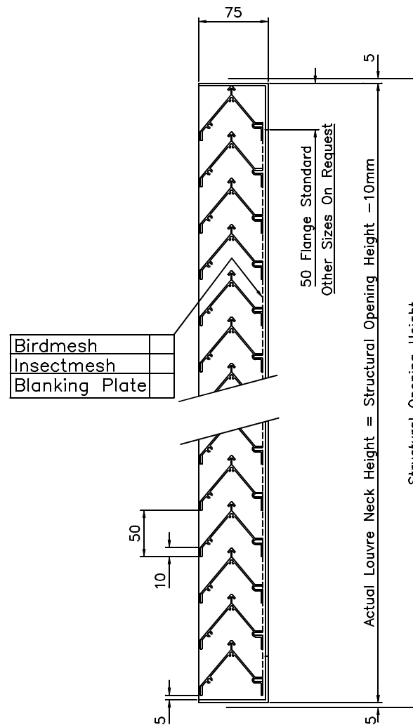
Sectional Plan On Arrow B.B.
