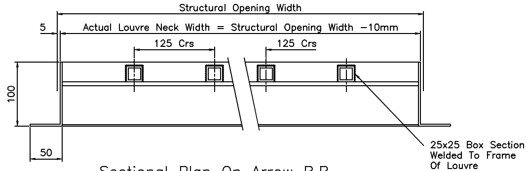
Sectional Plan On Arrow B.B.
