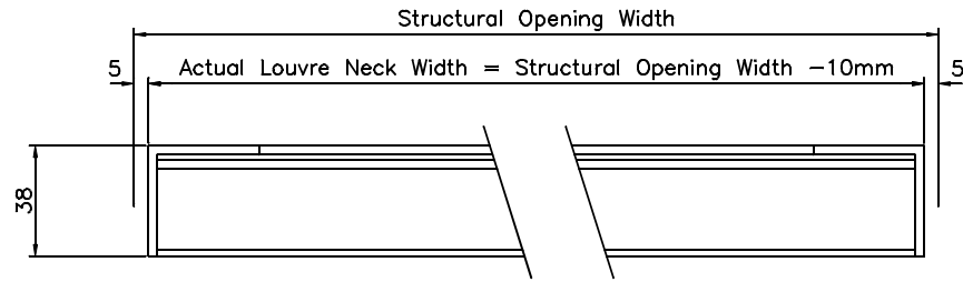
Sectional Plan On Arrow B.B.
