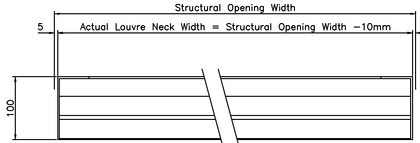
Sectional Plan On Arrow B.B.
