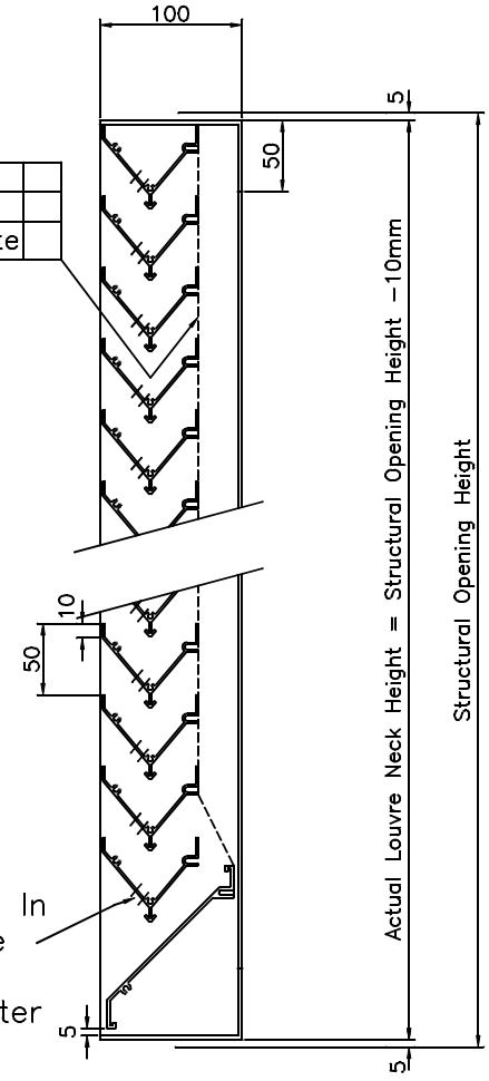
Sectional Elevation On Arrow A.A.
