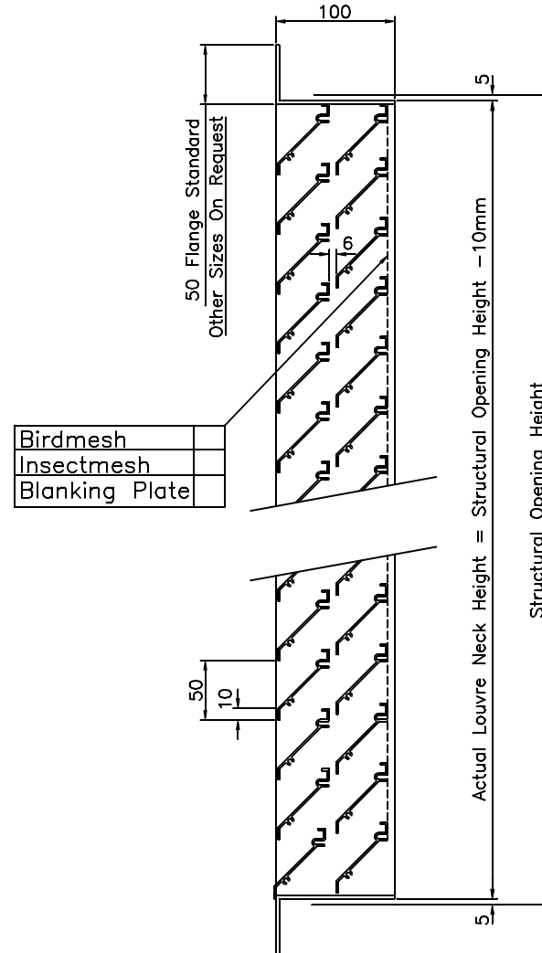
Sectional Elevation On Arrow A.A.
