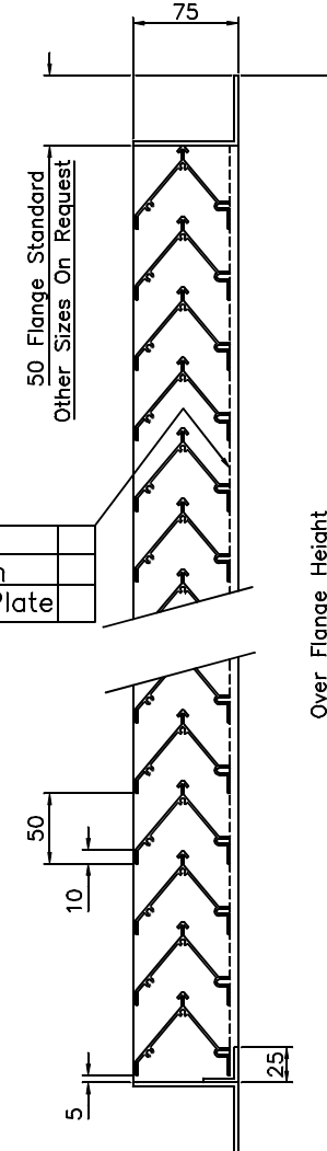
Sectional Elevation On Arrow A.A.
