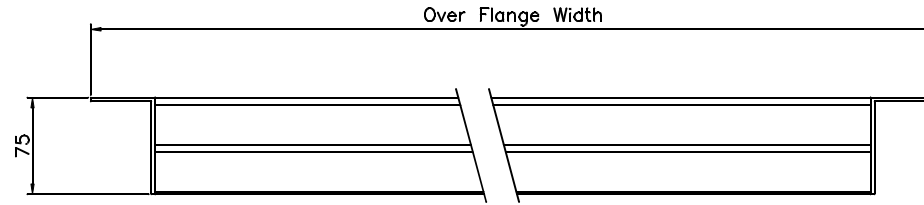
Sectional Plan On Arrow B.B.
