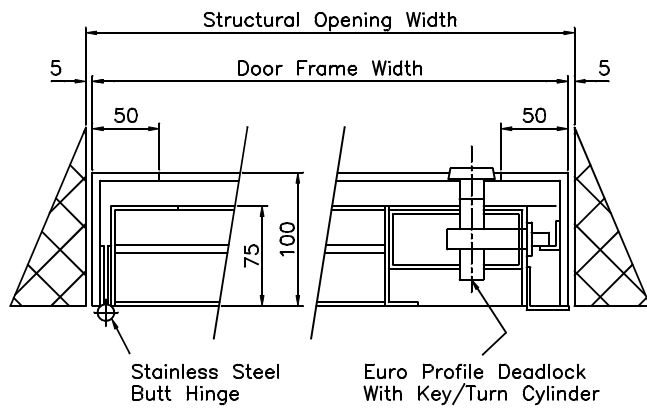
PLAN Section On B.B
