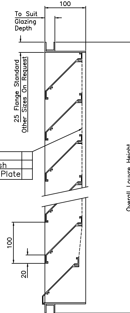
Sectional Elevation On Arrow A.A.
