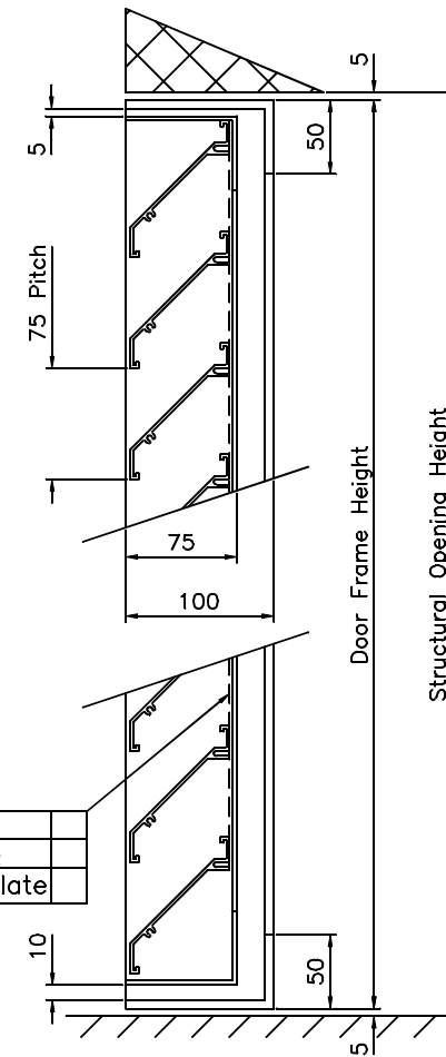
Sectional Side Elevation On A.A
