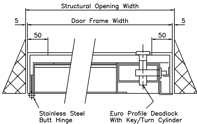
PLAN Section On B.B
