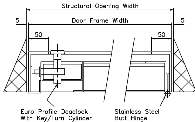
PLAN Section On C.C
