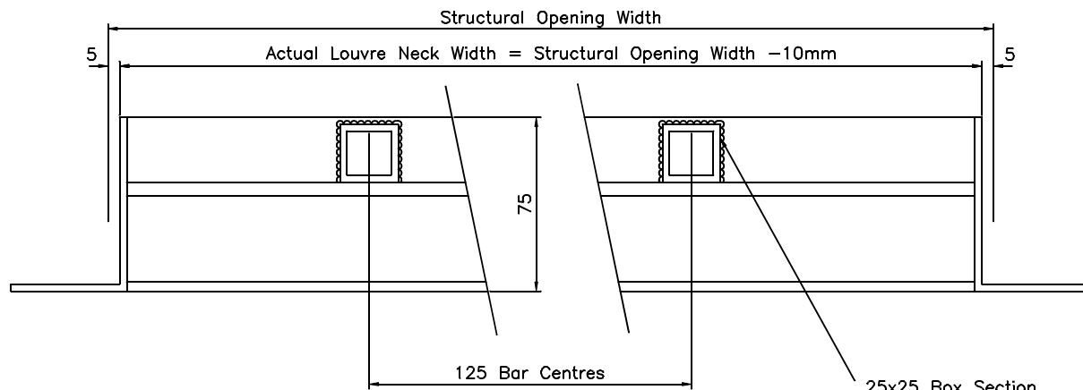
Sectional Plan On Arrow B.B.
