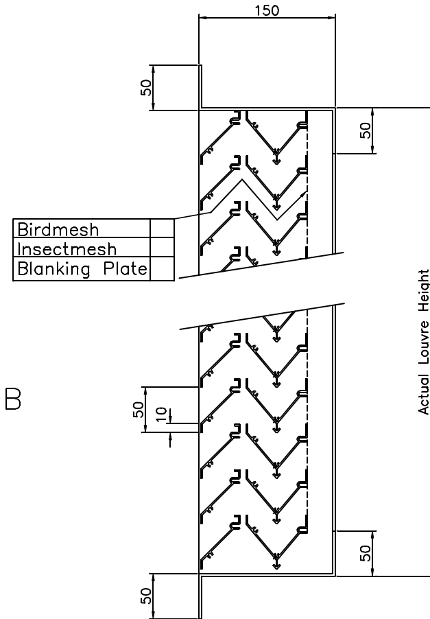
Sectional Elevation On Arrow A.A.
